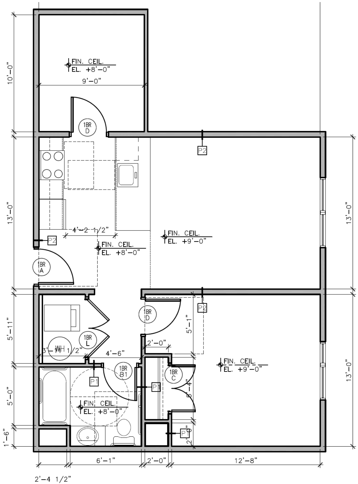
Typical one – bedroom, 1 bath unit (10 total units of this type in the building)
